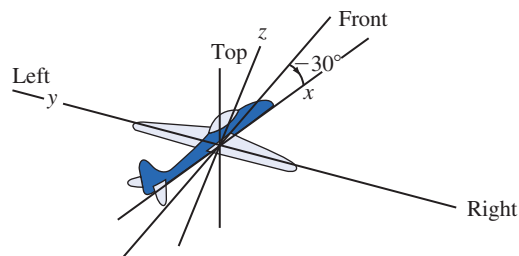
(c) Pitch of -30^\circ
