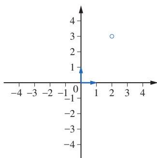
Terminal point of first vector (1, 0) Terminal point of second vector (0, 1) Target point (2, 3)
